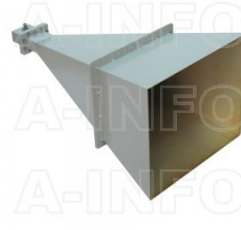
LB-340-20-C-NF Standard Gain Horn Antenna 2.2-3.3GHz 20dB Gain N Type Female
